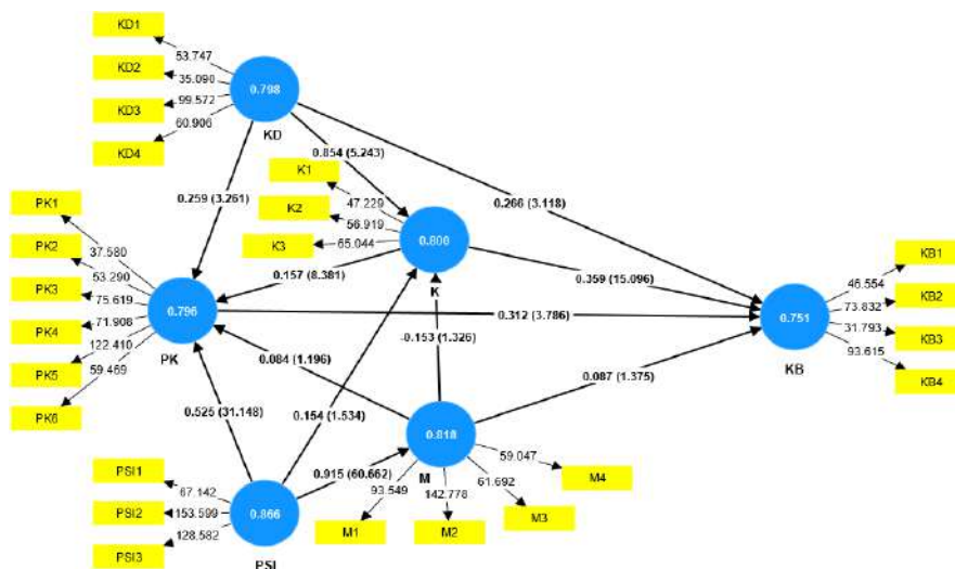
Figure 3. Bootstrapping SEM-PLS
