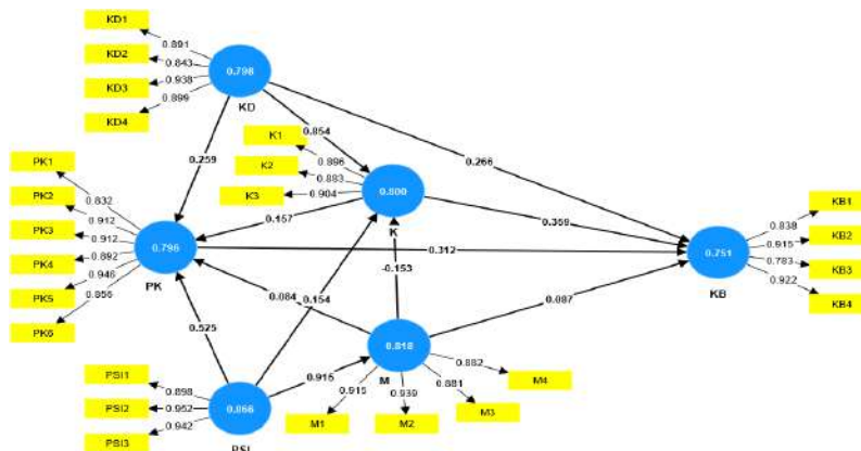
Figure 2. SEM-PLS Algorithm
