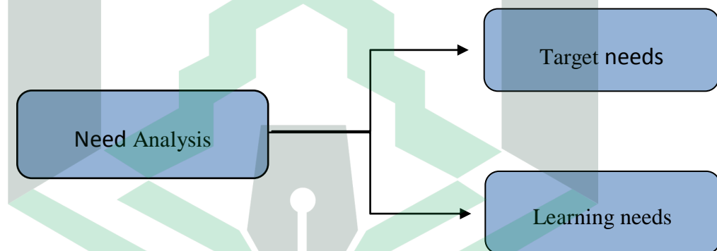
Figure 2.1 Theoretical Framework
